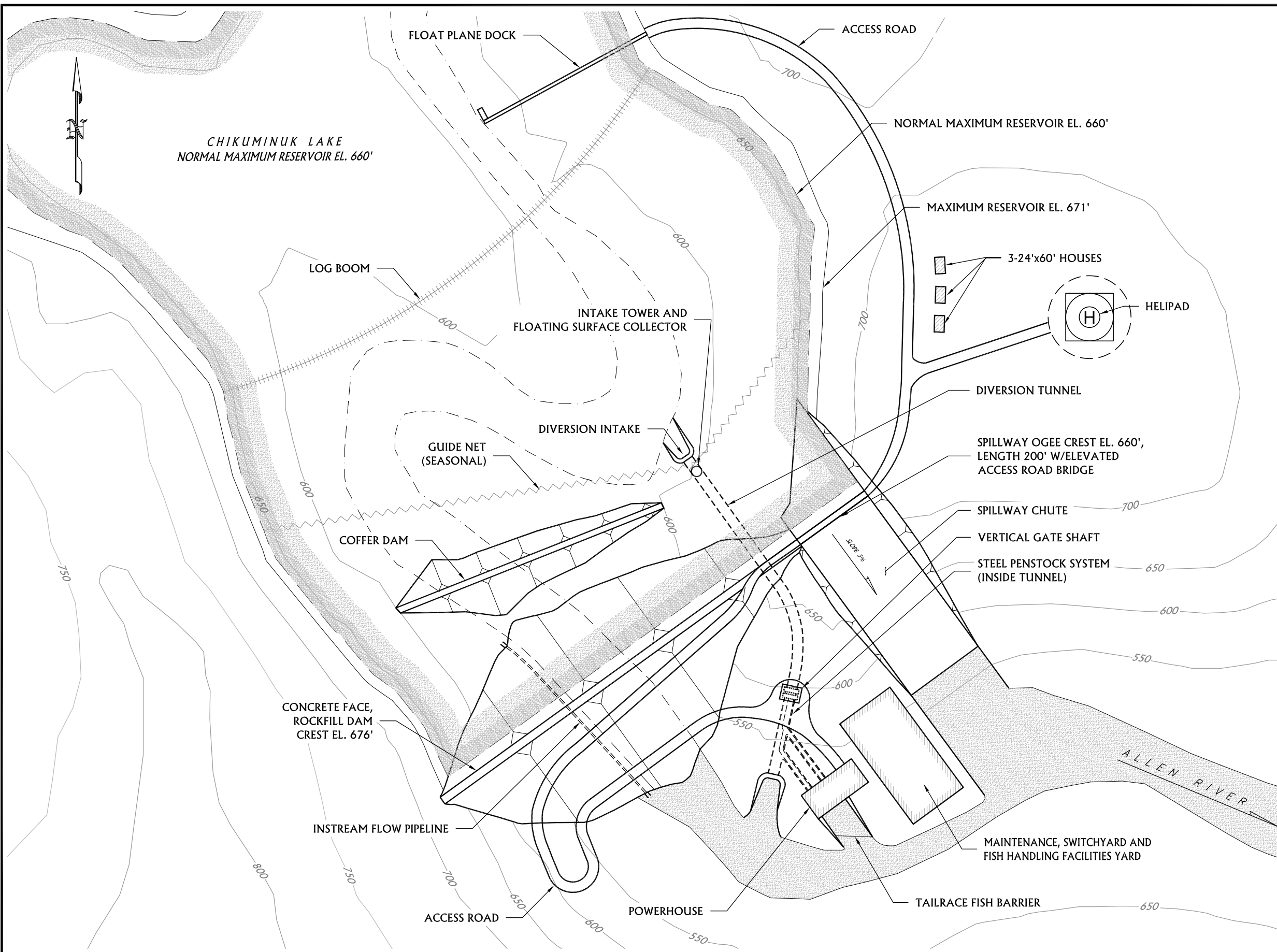
SITE PLAN
